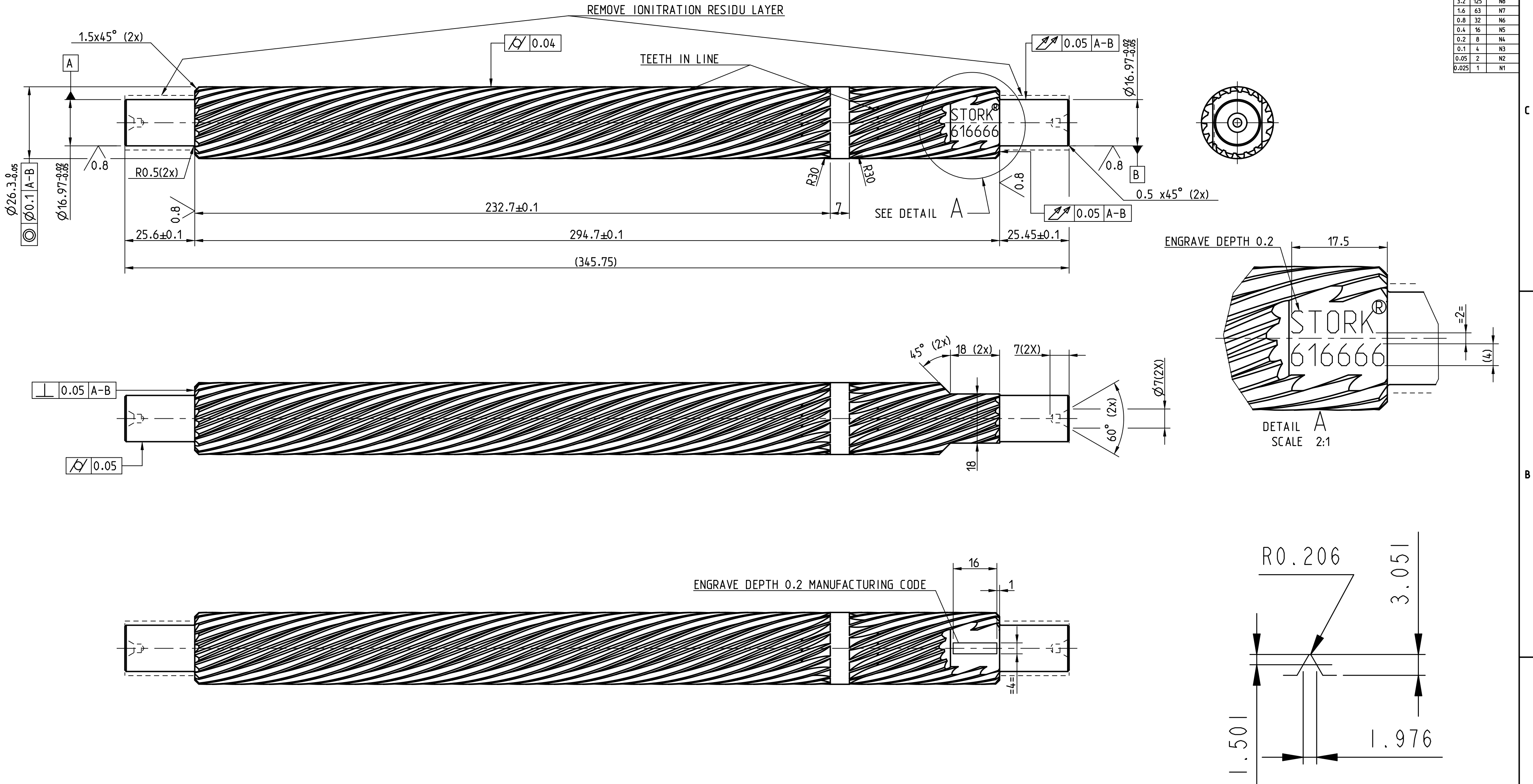
GEAR DESCRIPTION AFTER SURFACE FINISH
